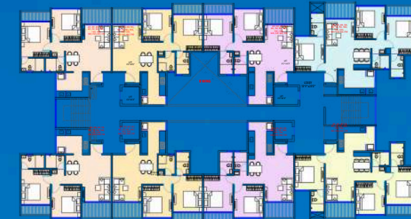
B WING KEY PLAN
